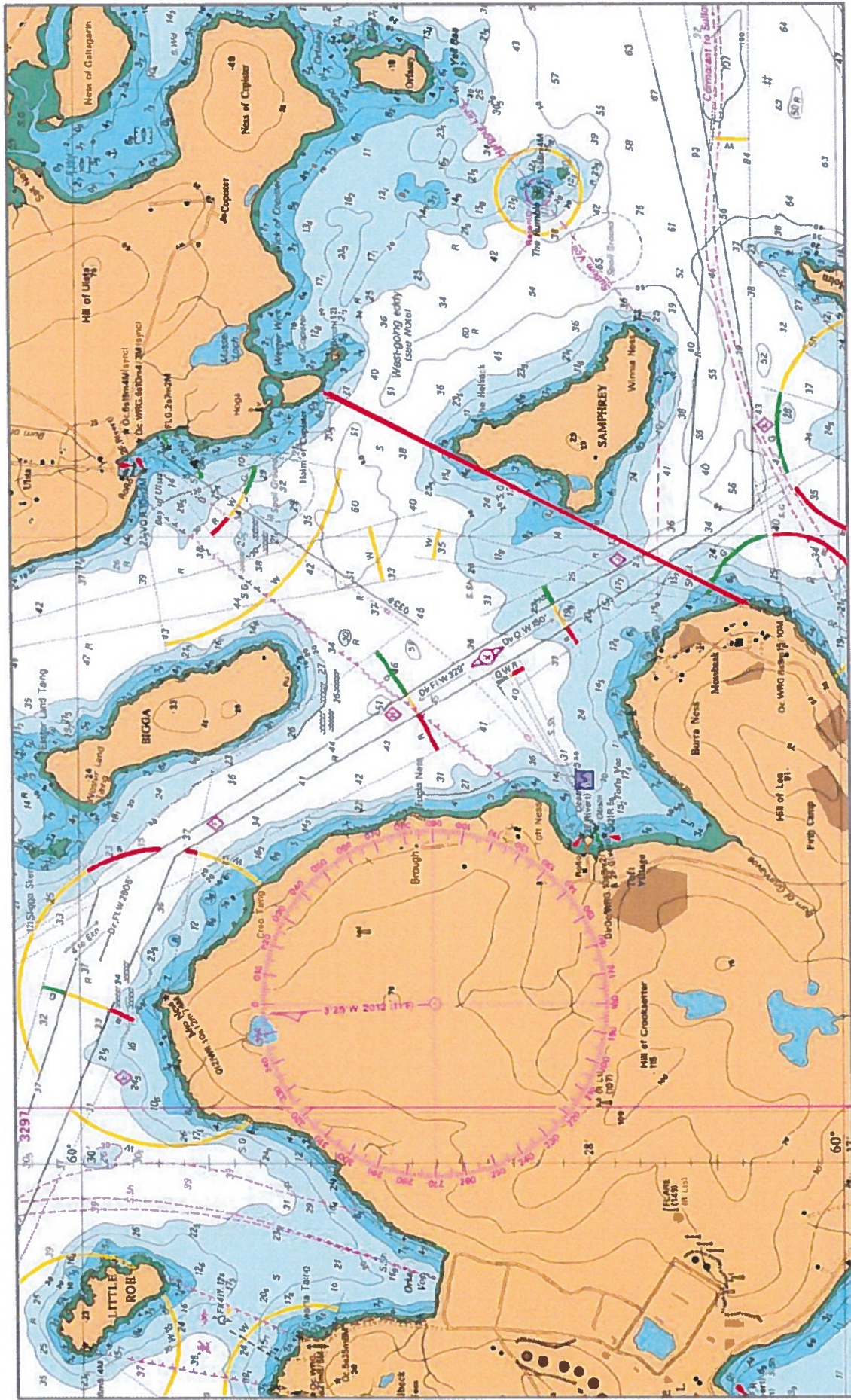
Figure 1 – Mossbank to Yell (South) Admiralty Chart
